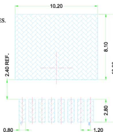
Land Pattern (Only For Reference)
